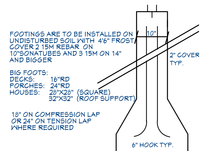
FOOTINGS & SONOTUBES TYP. Scale 1 - 12
