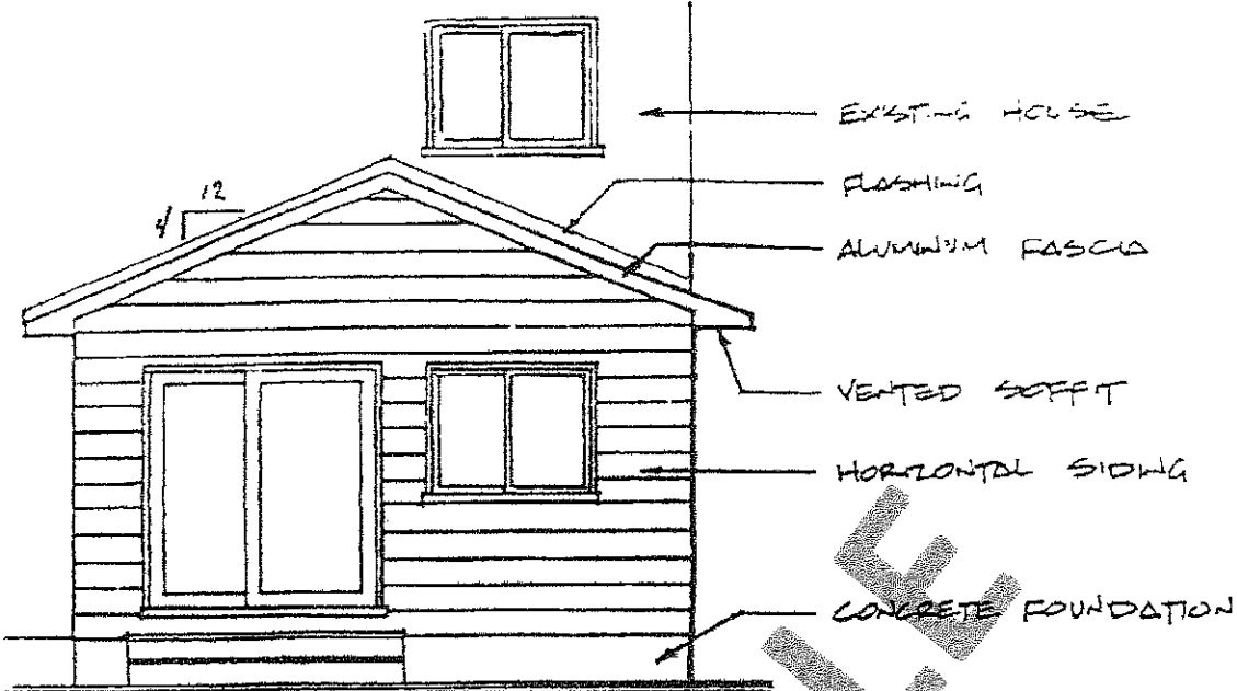
REAR ELEVATION SCALE = \frac{1}{4}'' = 1'-0''
