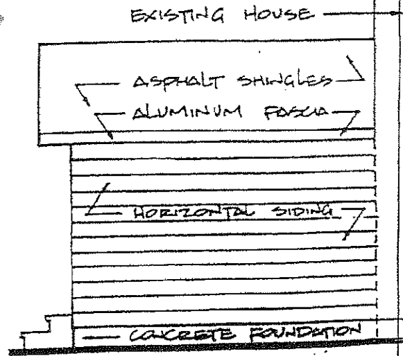
SIDE ELEVATION SCALE = \frac{1}{4}'' = 1'-0''
